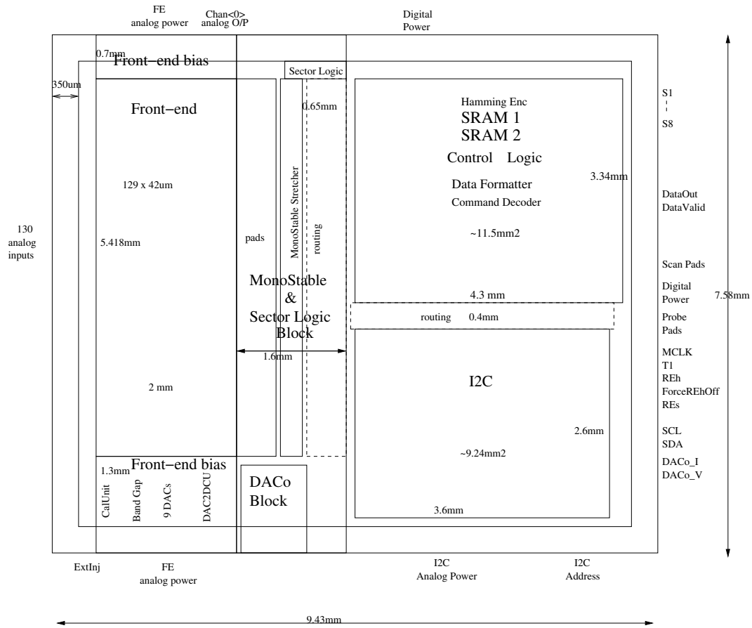
Figure 13: VFAT2 floorplan
