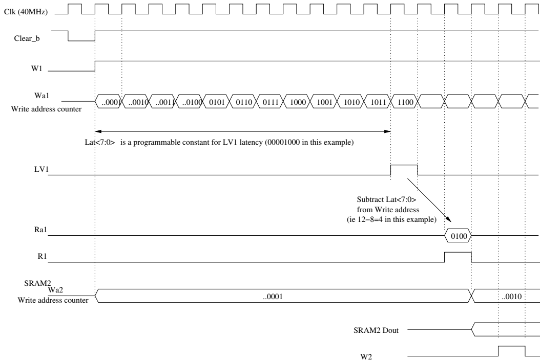
Figure 7: Timing diagram for the Write State Machine.
