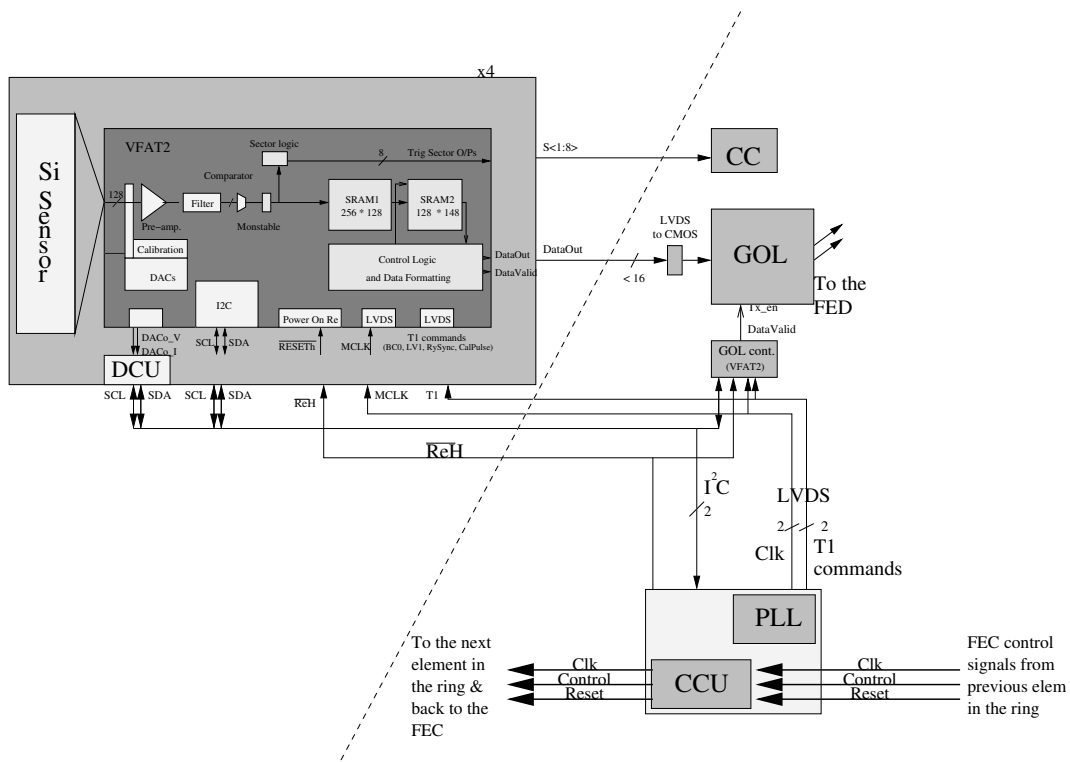
Figure 1: Block diagram of the Totem electronic system.
