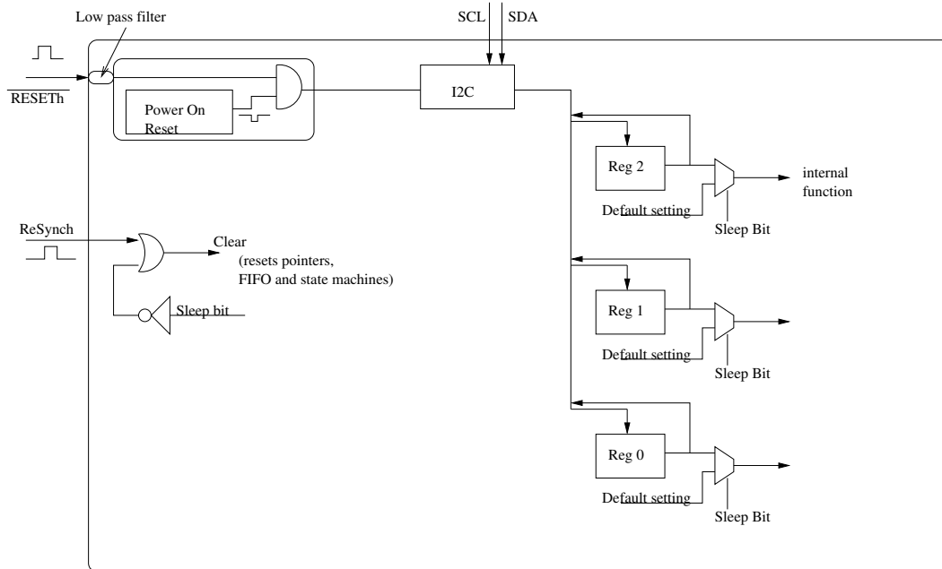
Figure 4: A schematic view of the programmable registers.
